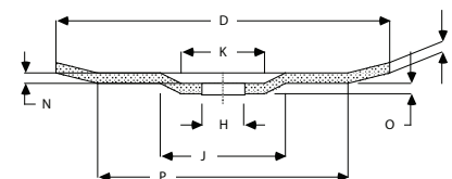
Type 28, Raised Hub Dish Wheel
