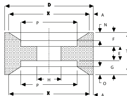
Type 26, Relieved and Recessed 2 sides
