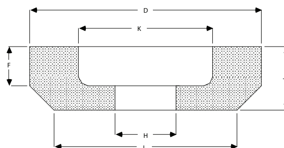
Type 6 Select-O-Point Drill Grinder
