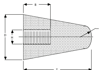
Type 17R Cone
