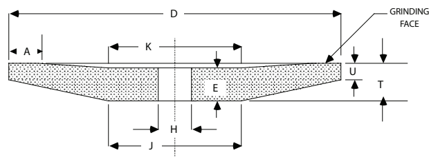
Type 12 Dish Wheels
