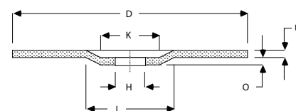
Type 27, Raised Hub Disc Wheel
