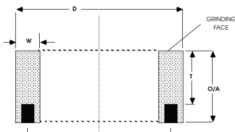
Type 52 Nut Inserted Cylinders
